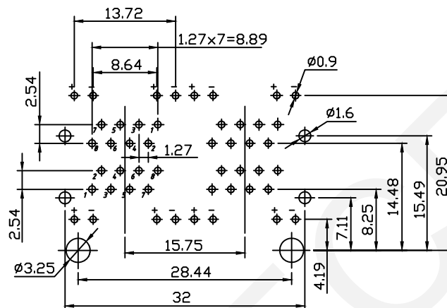
PCB Layout
